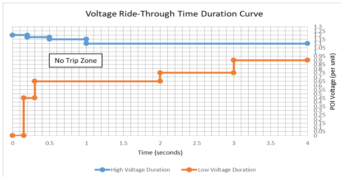
Graph 1: NERC Standard PRC-024 Voltage Ride-Through Requirements
